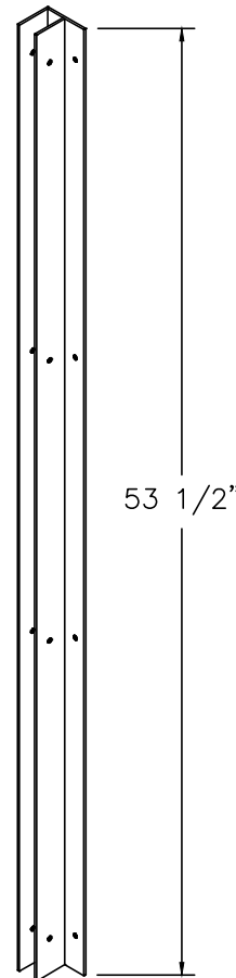
F BRACKET (PILASTER)
